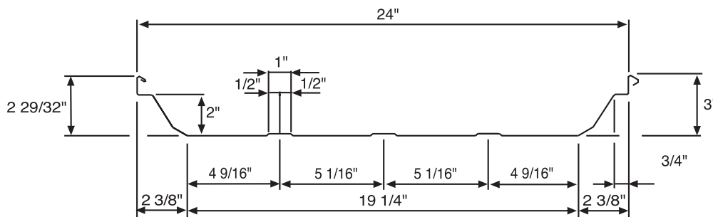
CROSS SECTION
